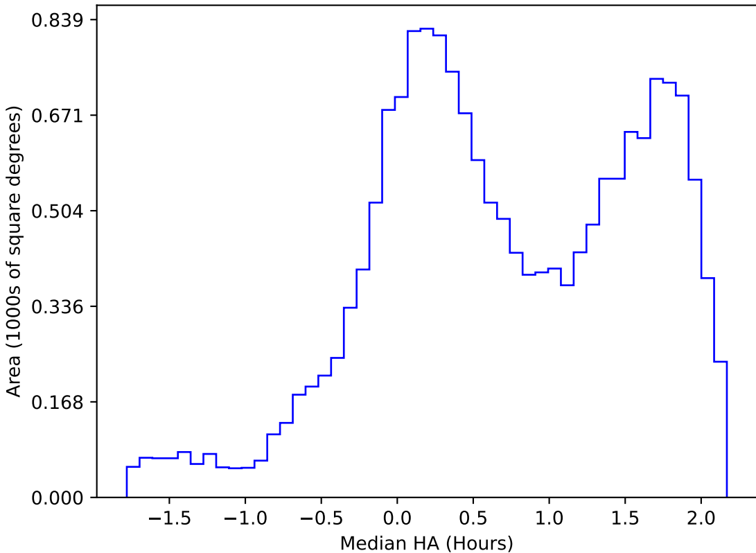
internal_u_expt27_nscale0.9v3.4_10yrs WFD g band: Median HA
