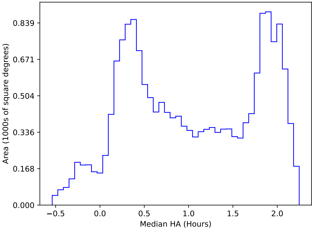
internal_u_expt27_nscale0.9v3.4_10yrs WFD all bands: Median HA
