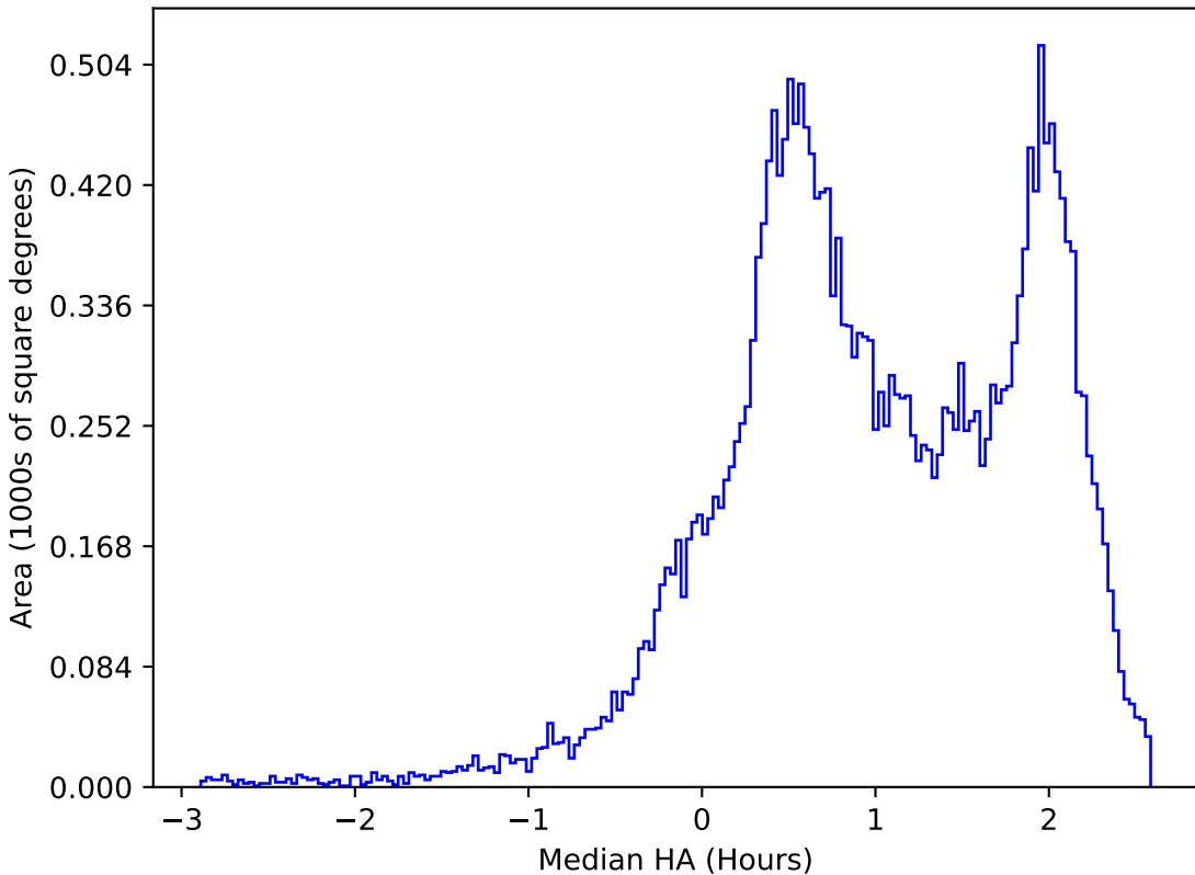
internal_u_expt27_nscale0.9v3.4_10yrs All sky z band: Median HA
