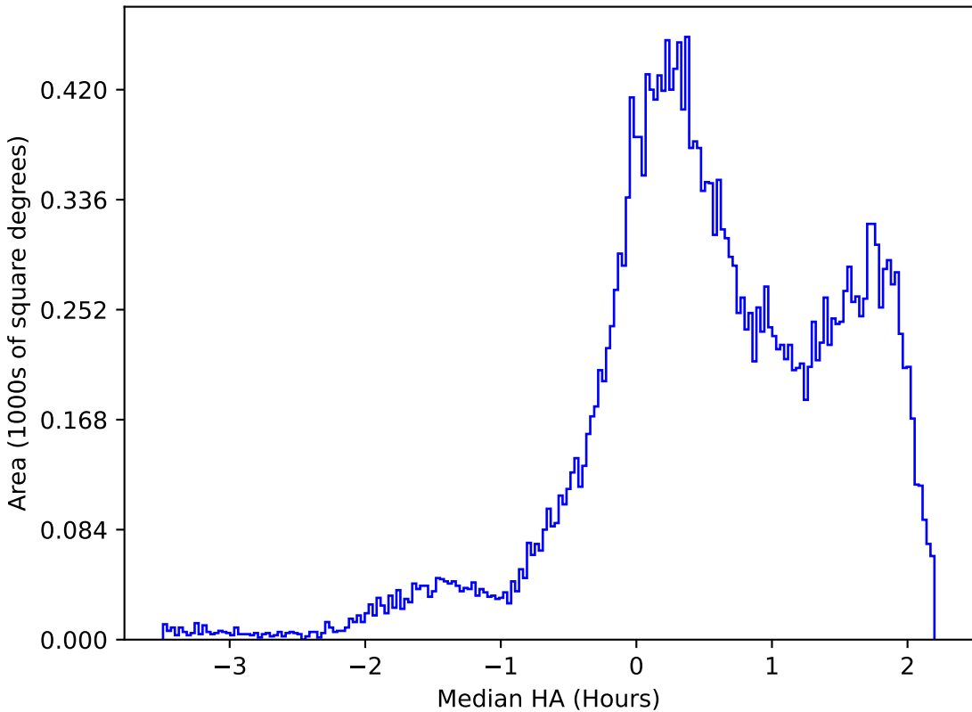
internal_u_expt27_nscale0.9v3.4_10yrs All sky g band: Median HA
