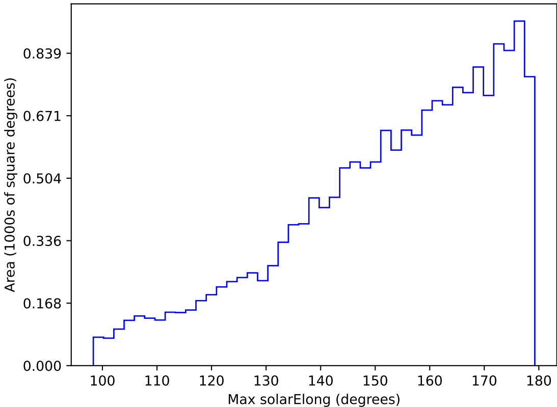
internal_u_expt27_nscale0.9v3.4_10yrs WFD g band: Max solarElong
