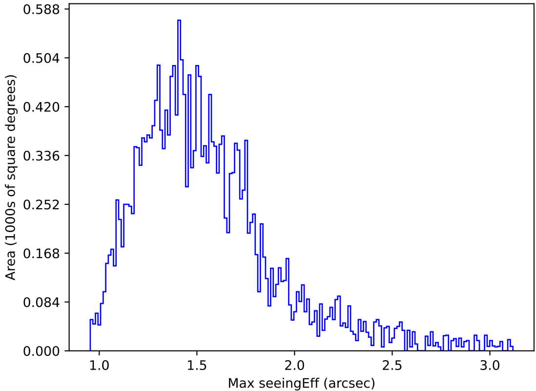
internal_u_expt27_nscale0.9v3.4_10yrs Yr 1 u band: Max seeingEff
