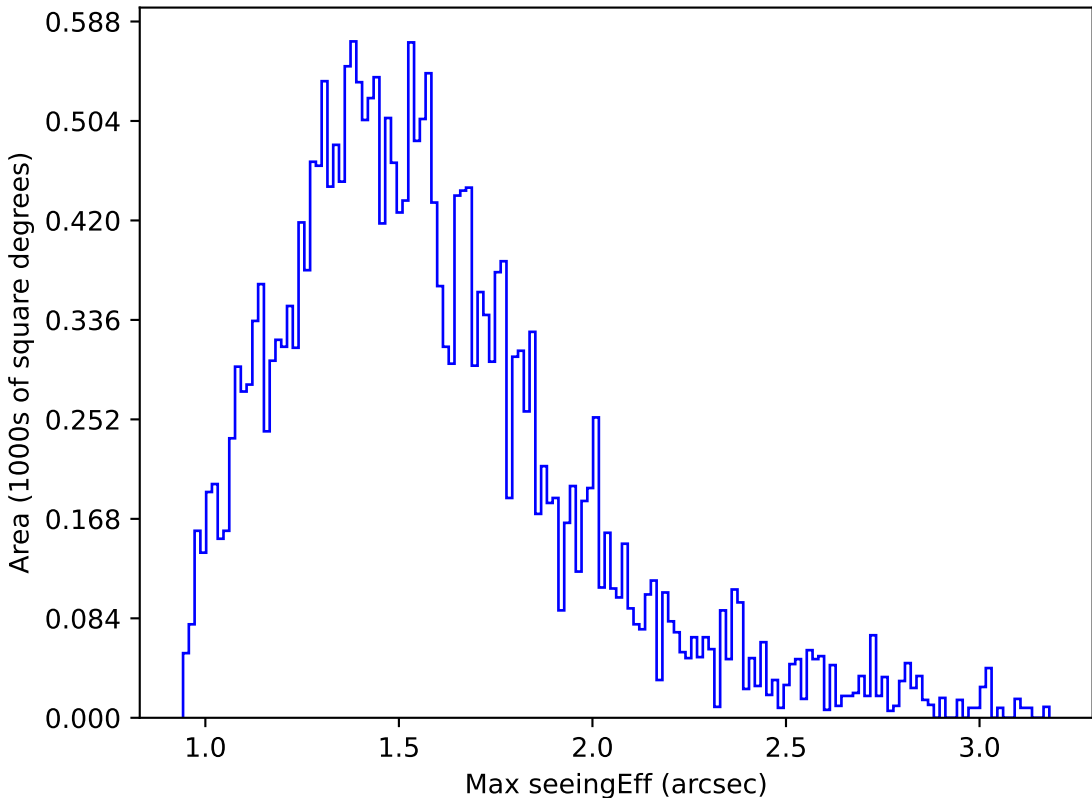
internal_u_expt27_nscale0.9v3.4_10yrs Yr 1 i band: Max seeingEff
