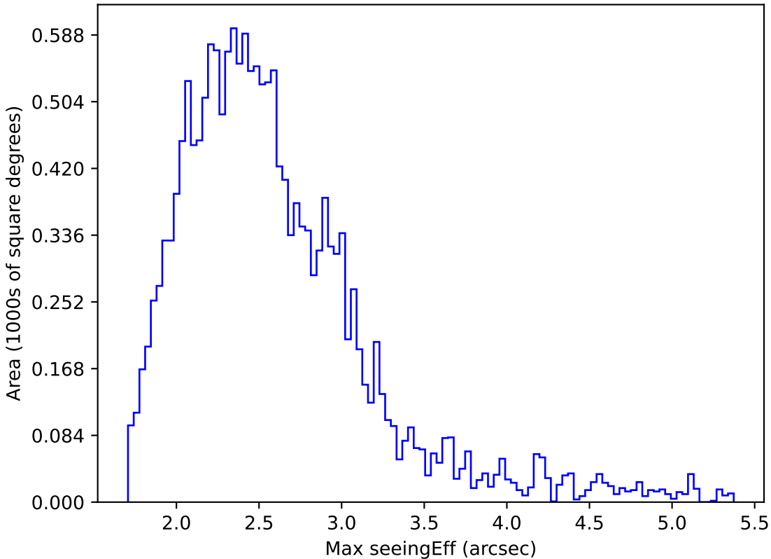
internal_u_expt27_nscale0.9v3.4_10yrs WFD z band: Max seeingEff
