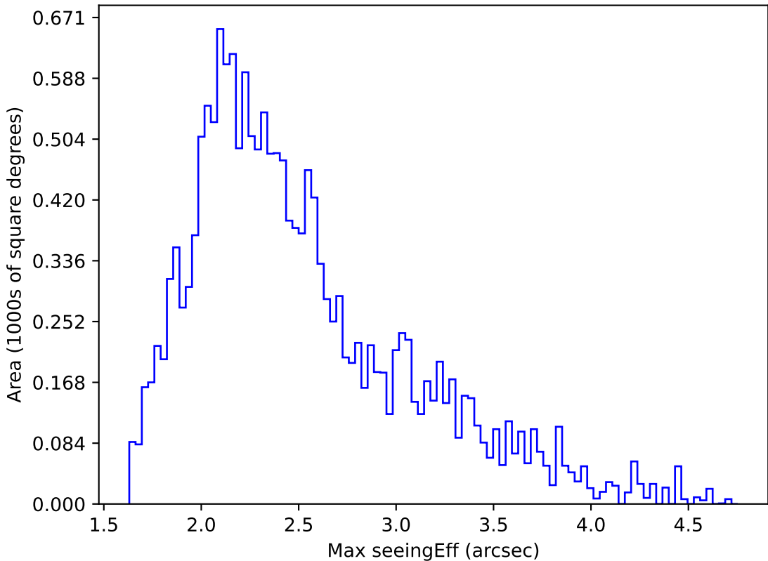
internal_u_expt27_nscale0.9v3.4_10yrs WFD u band: Max seeingEff
