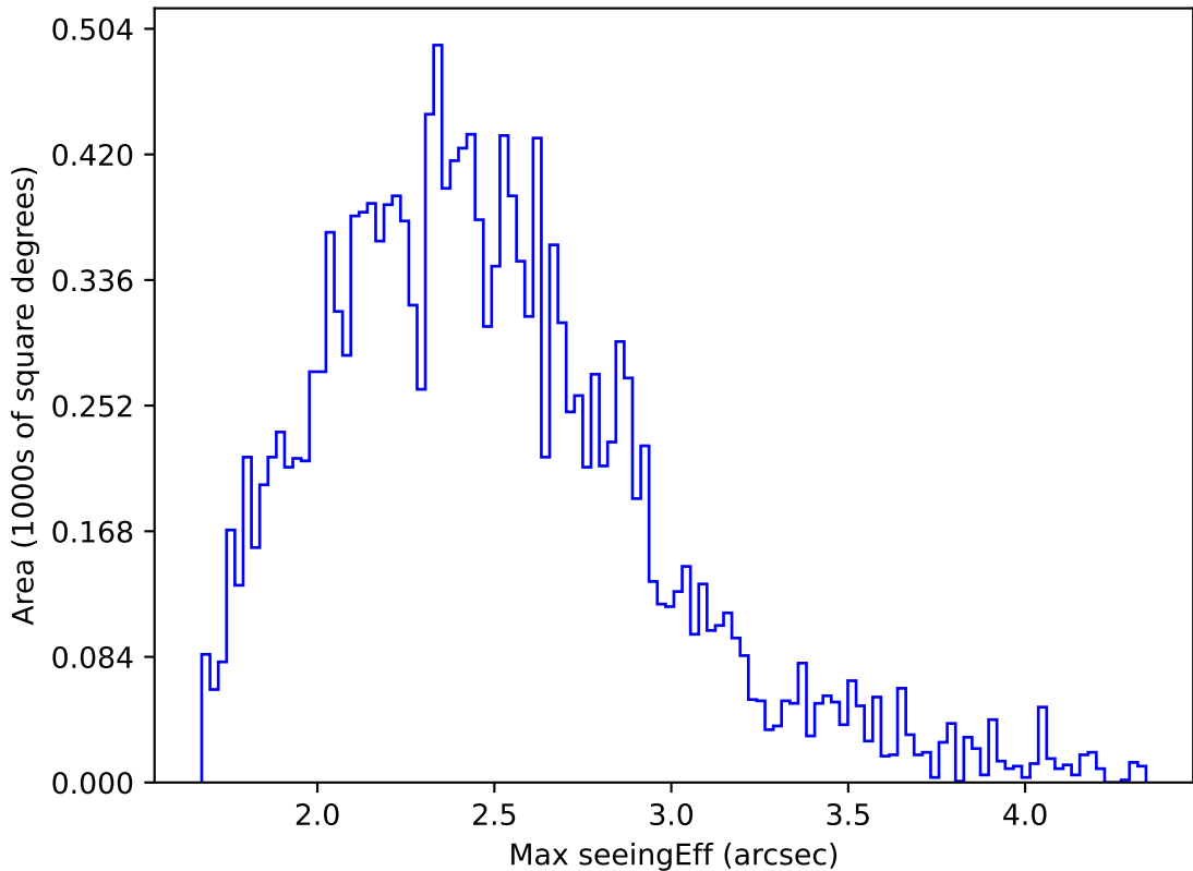
internal_u_expt27_nscale0.9v3.4_10yrs WFD g band: Max seeingEff
