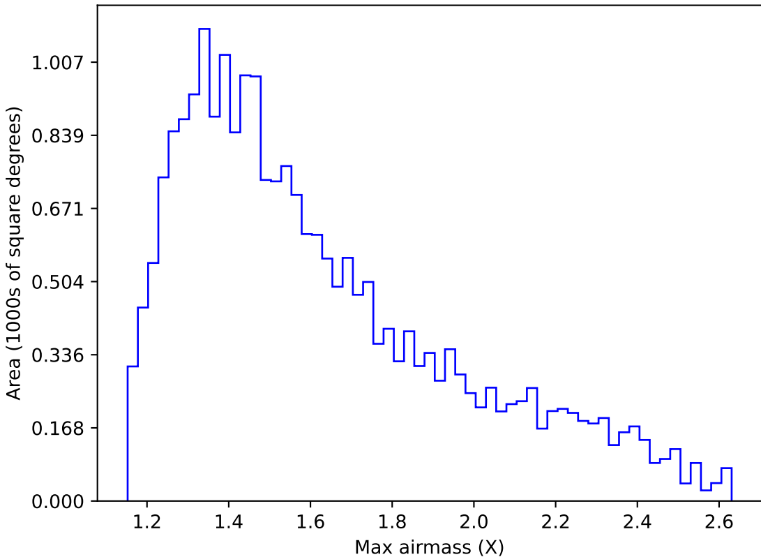
internal_u_expt27_nscale0.9v3.4_10yrs Yr 1 y band: Max airmass
