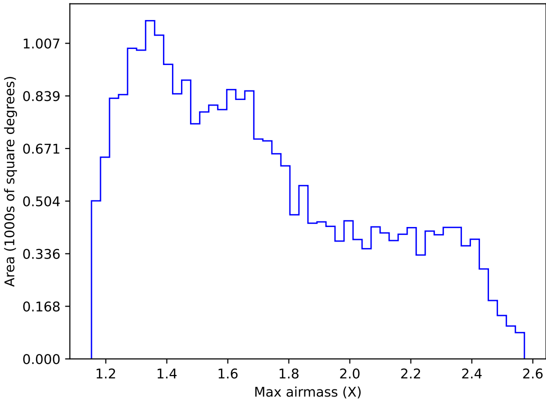
internal_u_expt27_nscale0.9v3.4_10yrs Yr 1 r band: Max airmass
