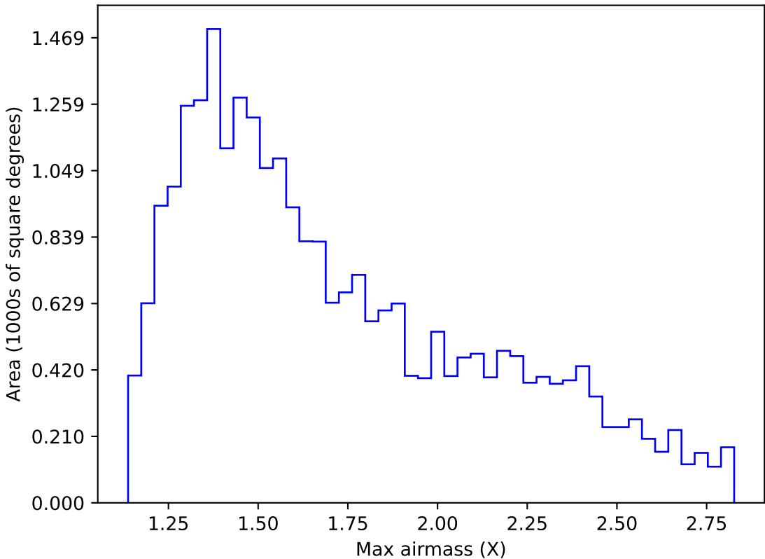
internal_u_expt27_nscale0.9v3.4_10yrs Yr 1 i band: Max airmass
