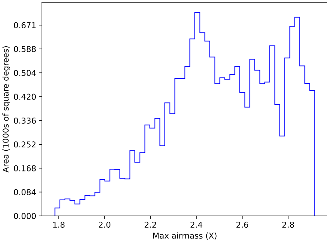
internal_u_expt27_nscale0.9v3.4_10yrs WFD z band: Max airmass
