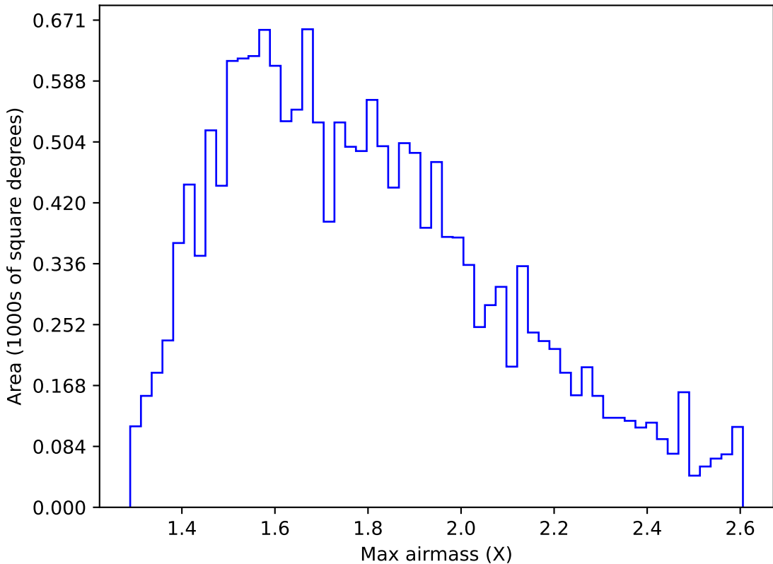
internal_u_expt27_nscale0.9v3.4_10yrs WFD u band: Max airmass
