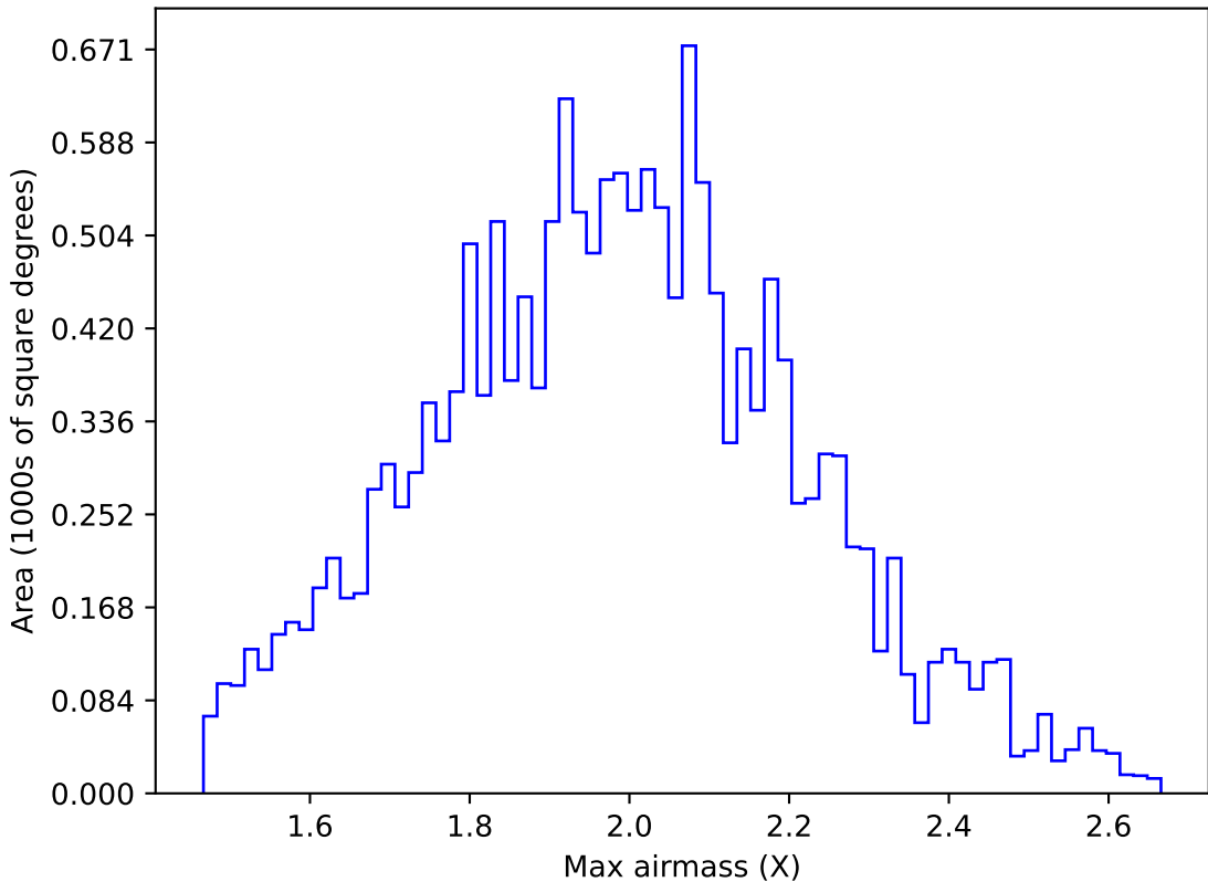
internal_u_expt27_nscale0.9v3.4_10yrs WFD g band: Max airmass
