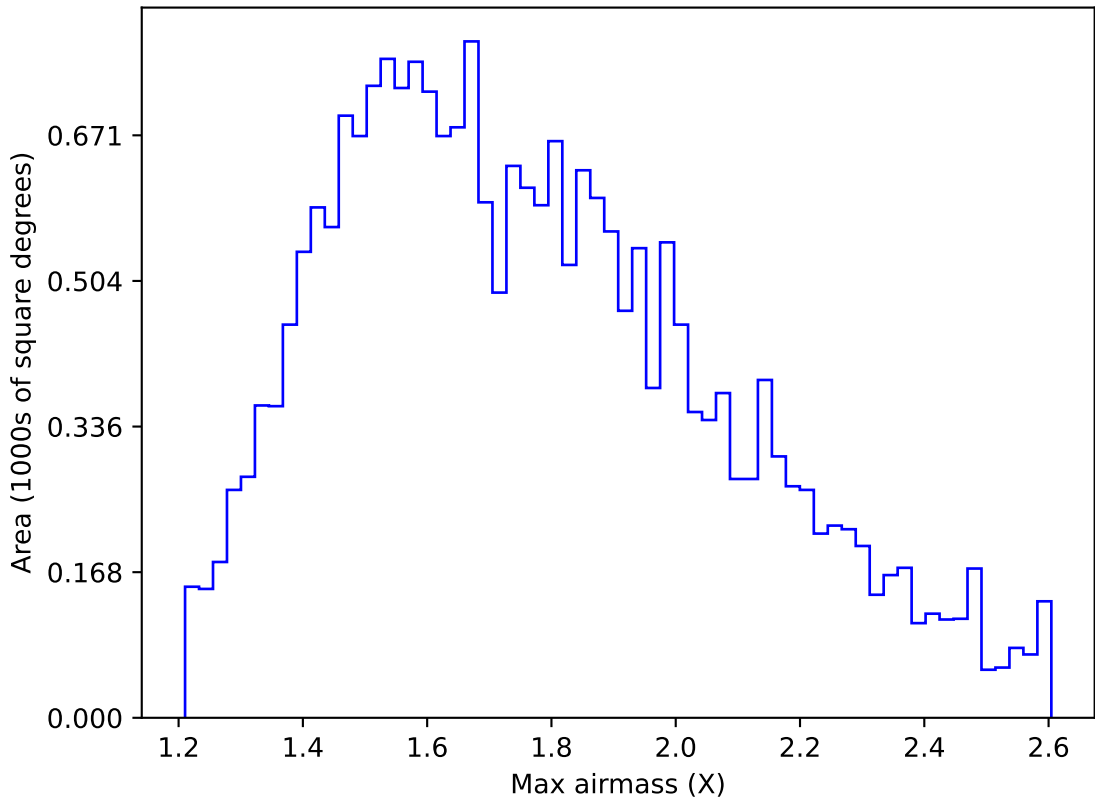
internal_u_expt27_nscale0.9v3.4_10yrs All sky u band: Max airmass
