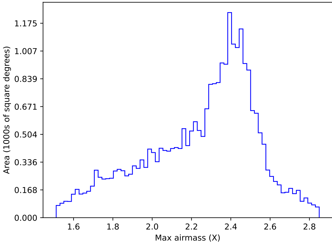
internal_u_expt27_nscale0.9v3.4_10yrs All sky r band: Max airmass
