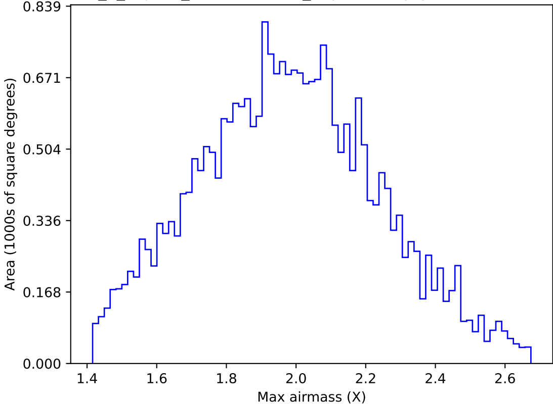
internal_u_expt27_nscale0.9v3.4_10yrs All sky g band: Max airmass
