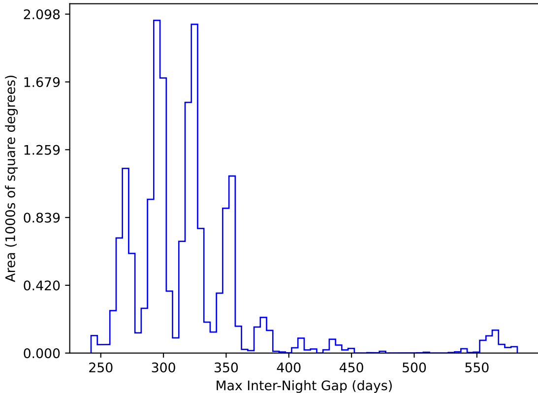
internal_u_expt27_nscale0.9v3.4_10yrs WFD y band: Max Inter-Night Gap
