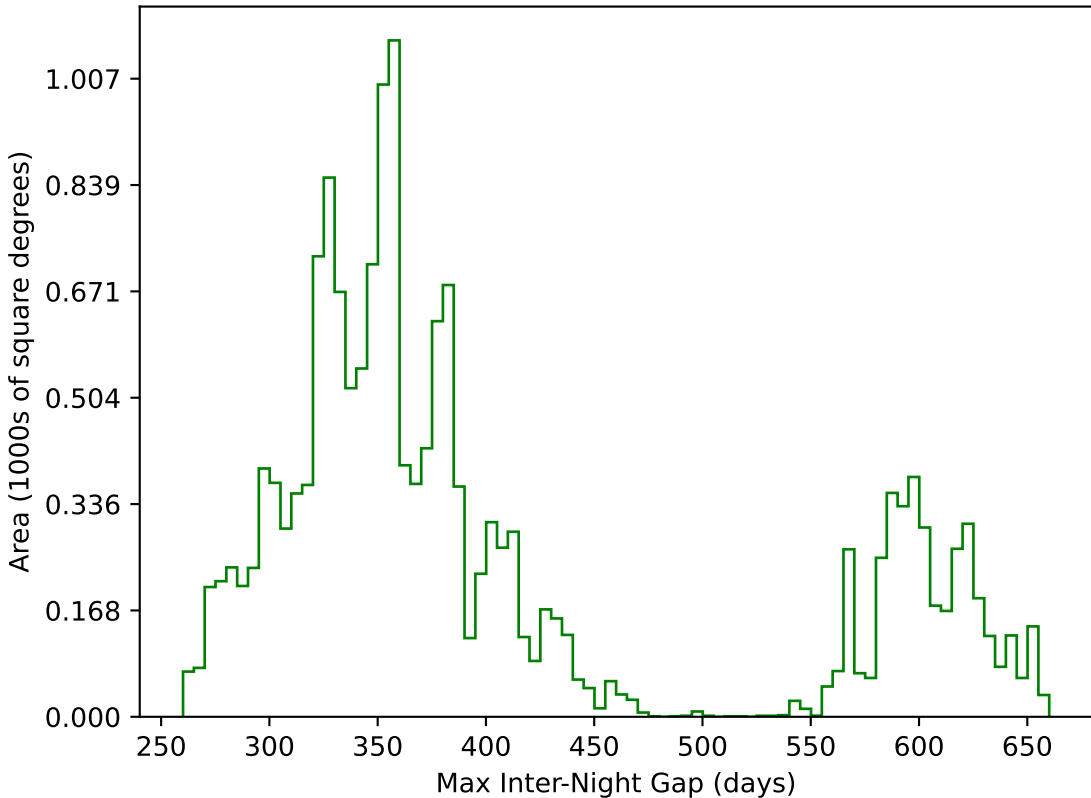
internal_u_expt27_nscale0.9v3.4_10yrs WFD g band: Max Inter-Night Gap
