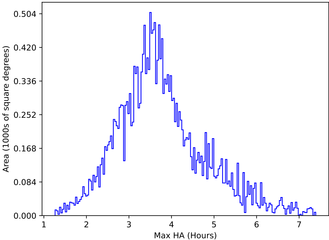
internal_u_expt27_nscale0.9v3.4_10yrs All sky u band: Max HA
