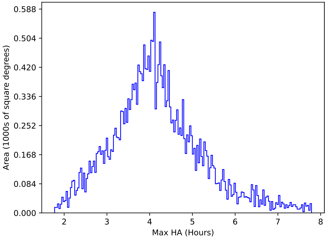
internal_u_expt27_nscale0.9v3.4_10yrs All sky r band: Max HA
