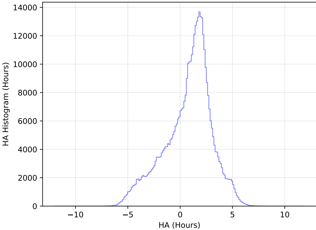
internal_u_expt27_nscale0.9v3.4_10yrs WFD z band: HA Histogram
