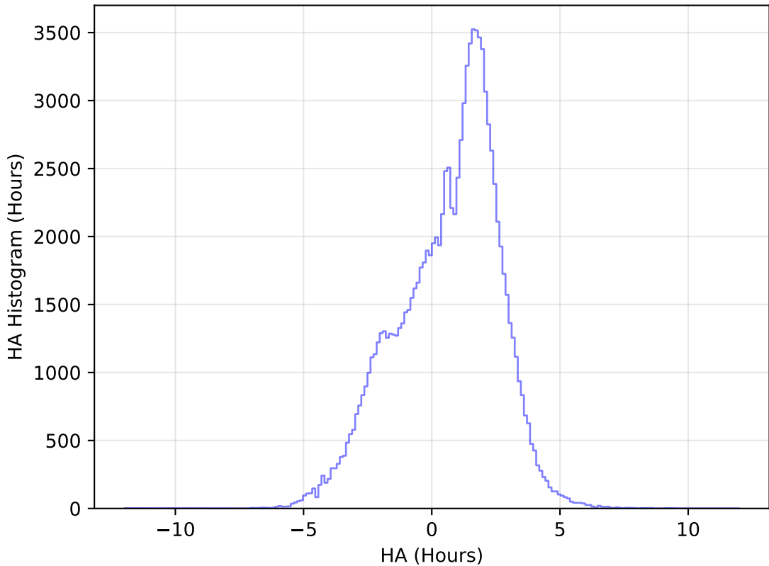
internal_u_expt27_nscale0.9v3.4_10yrs WFD u band: HA Histogram
