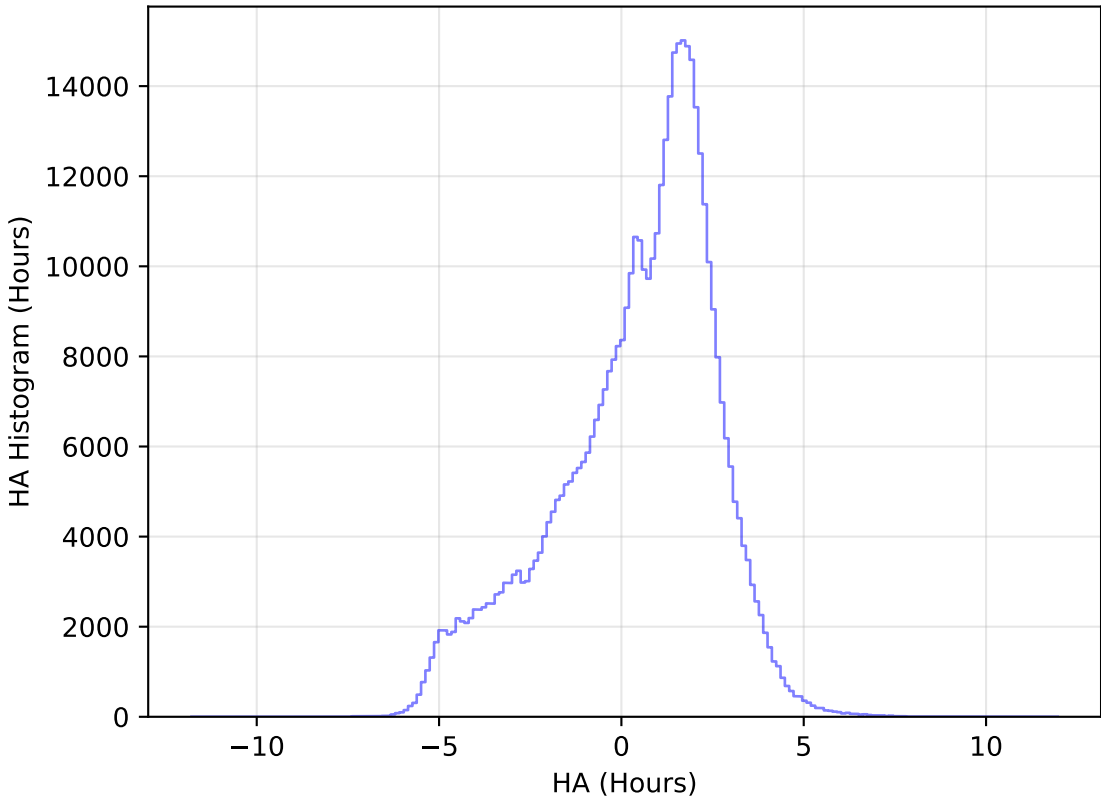
internal_u_expt27_nscale0.9v3.4_10yrs WFD r band: HA Histogram
