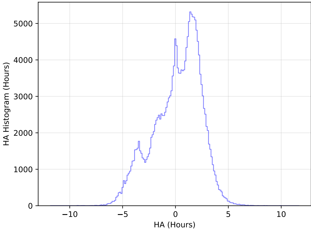
internal_u_expt27_nscale0.9v3.4_10yrs WFD g band: HA Histogram
