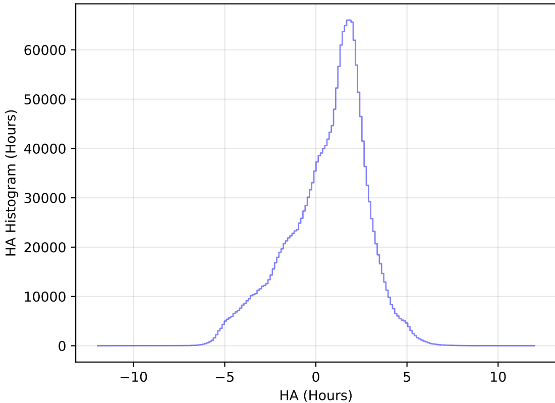
internal_u_expt27_nscale0.9v3.4_10yrs WFD all bands: HA Histogram
