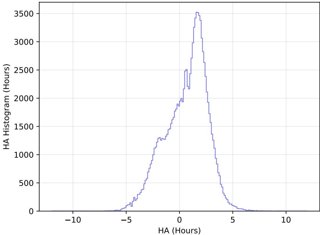
internal_u_expt27_nscale0.9v3.4_10yrs All sky u band: HA Histogram
