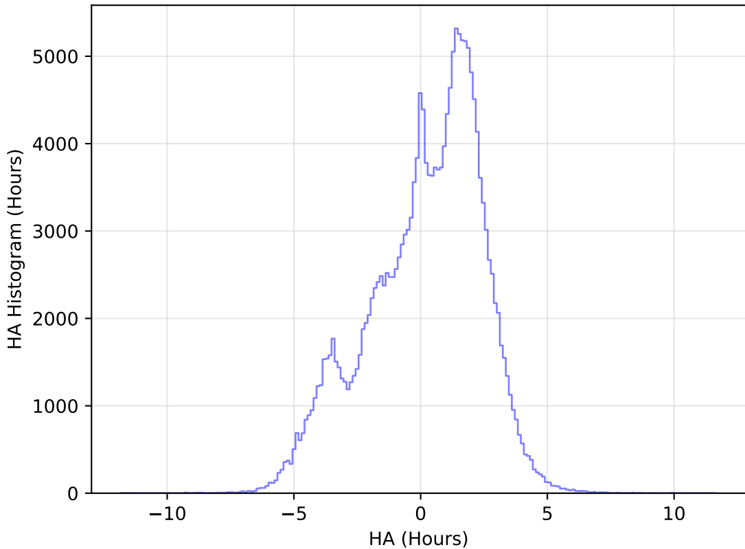
internal_u_expt27_nscale0.9v3.4_10yrs All sky g band: HA Histogram
