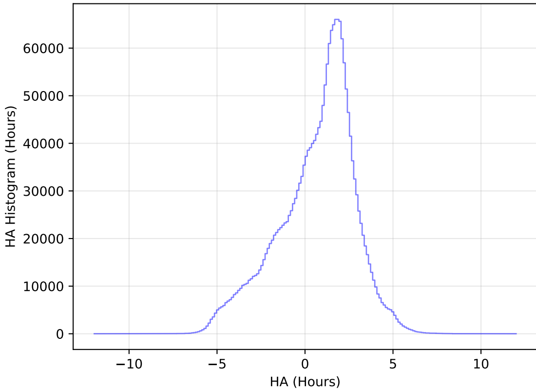
internal_u_expt27_nscale0.9v3.4_10yrs All sky all bands: HA Histogram
