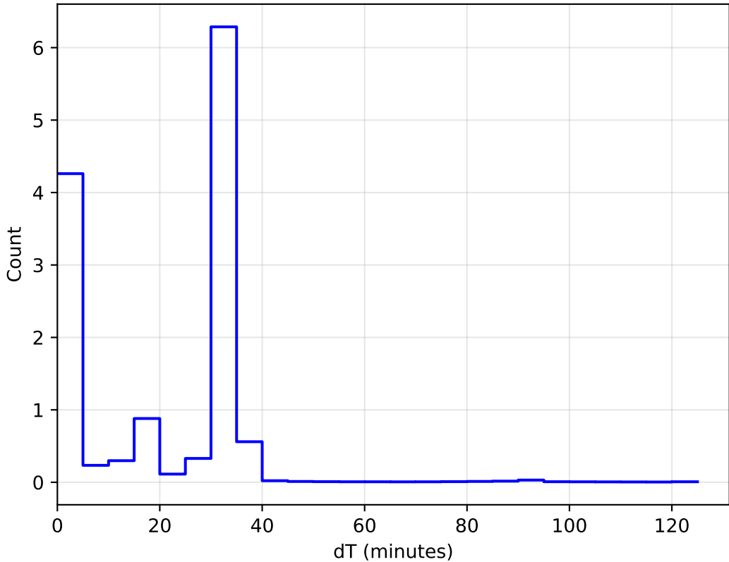
internal_u_expt27_nscale0.9v3.4_10yrs All sky: DeltaT Histogram
