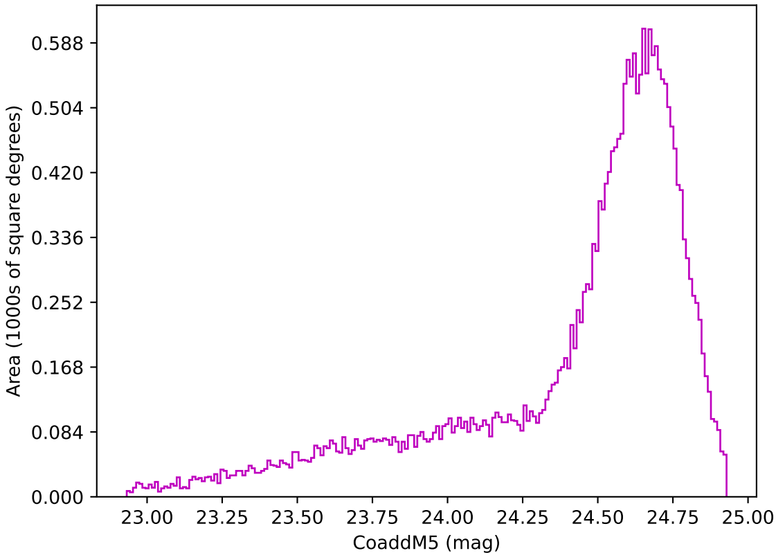
internal_u_expt27_nscale0.9v3.4_10yrs Yr 1 z band: CoaddM5
