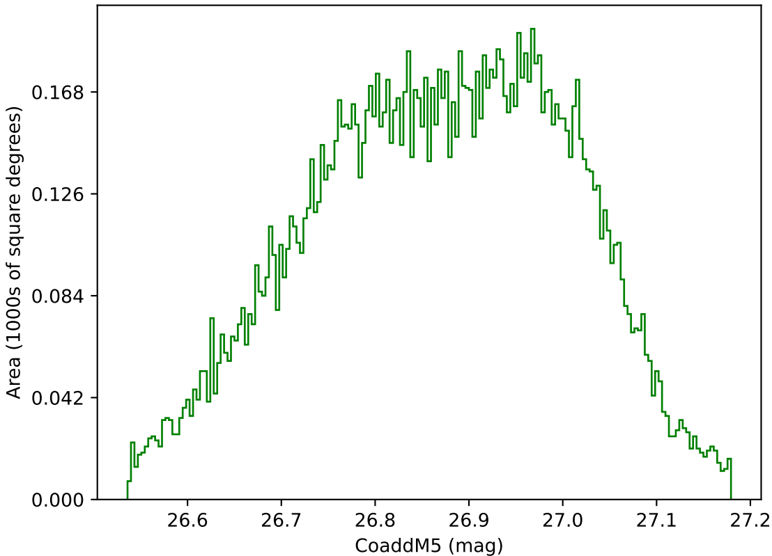
internal_u_expt27_nscale0.9v3.4_10yrs WFD g band: CoaddM5
