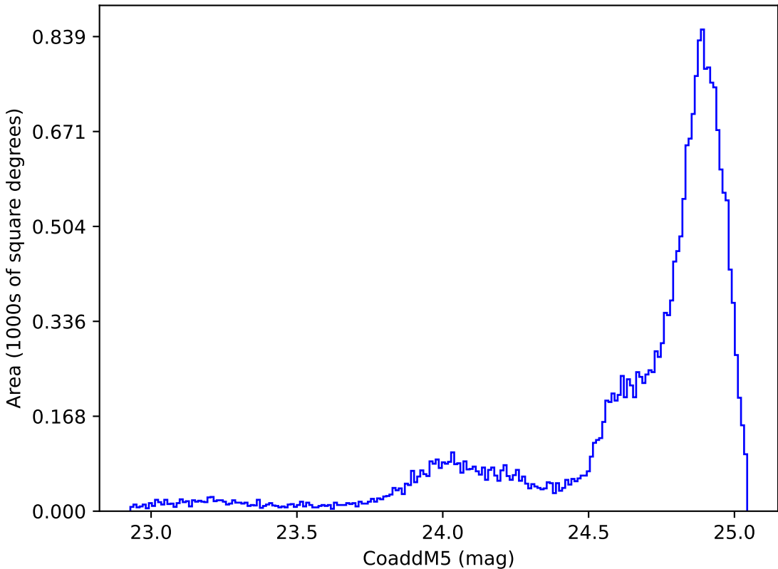
internal_u_expt27_nscale0.9v3.4_10yrs All sky y band: CoaddM5
