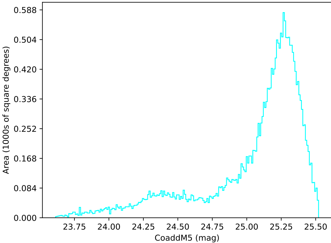
internal_u_expt27_nscale0.9v3.4_10yrs All sky u band: CoaddM5
