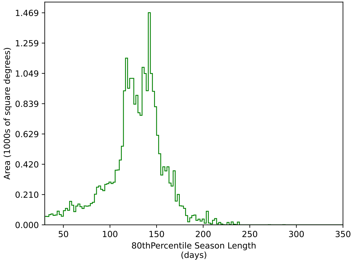
internal_u_expt27_nscale0.9v3.4_10yrs All sky g band: 80thPercentile Season Length
