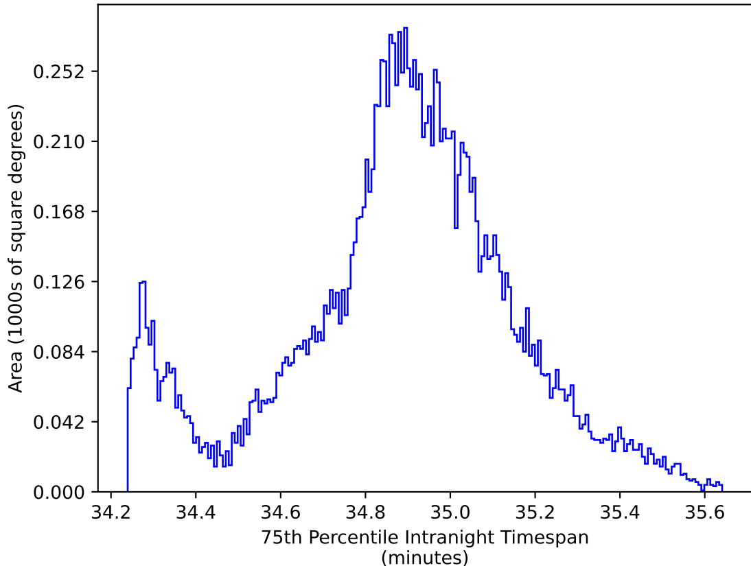
internal_u_expt27_nscale0.9v3.4_10yrs WFD all bands: 75th Percentile Intranight Timespan
