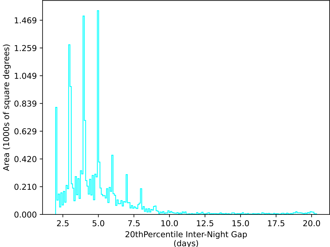
internal_u_expt27_nscale0.9v3.4_10yrs WFD u band: 20thPercentile Inter-Night Gap
