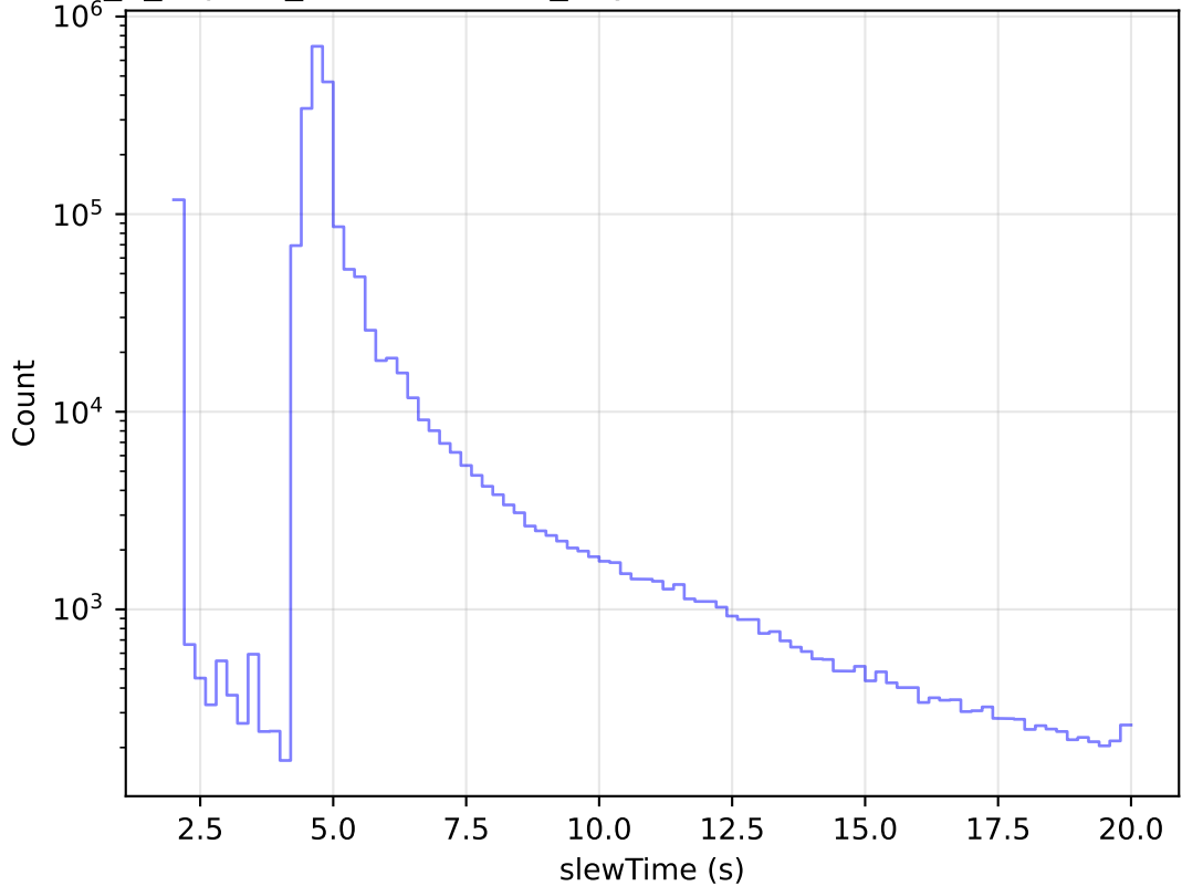
internal_u_expt27_nscale0.9v3.4_10yrs All visits: Zoom Slew Time Histogram
