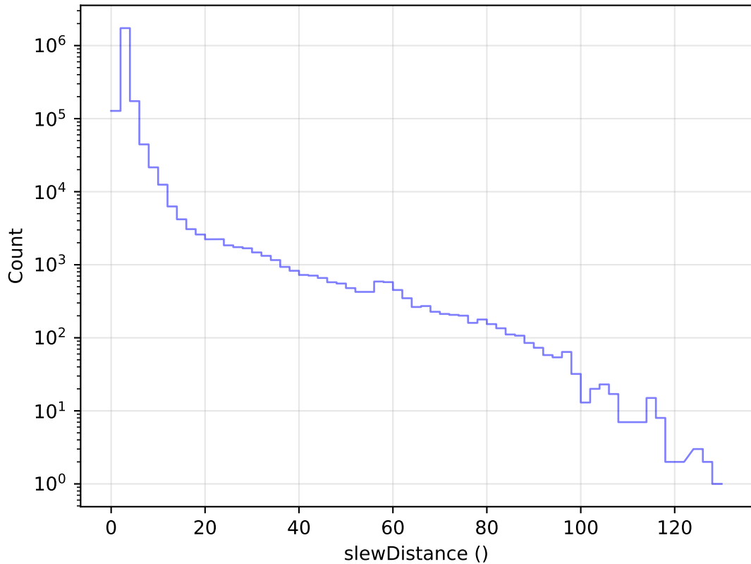
internal_u_expt27_nscale0.9v3.4_10yrs All visits: Slew Distance Histogram
