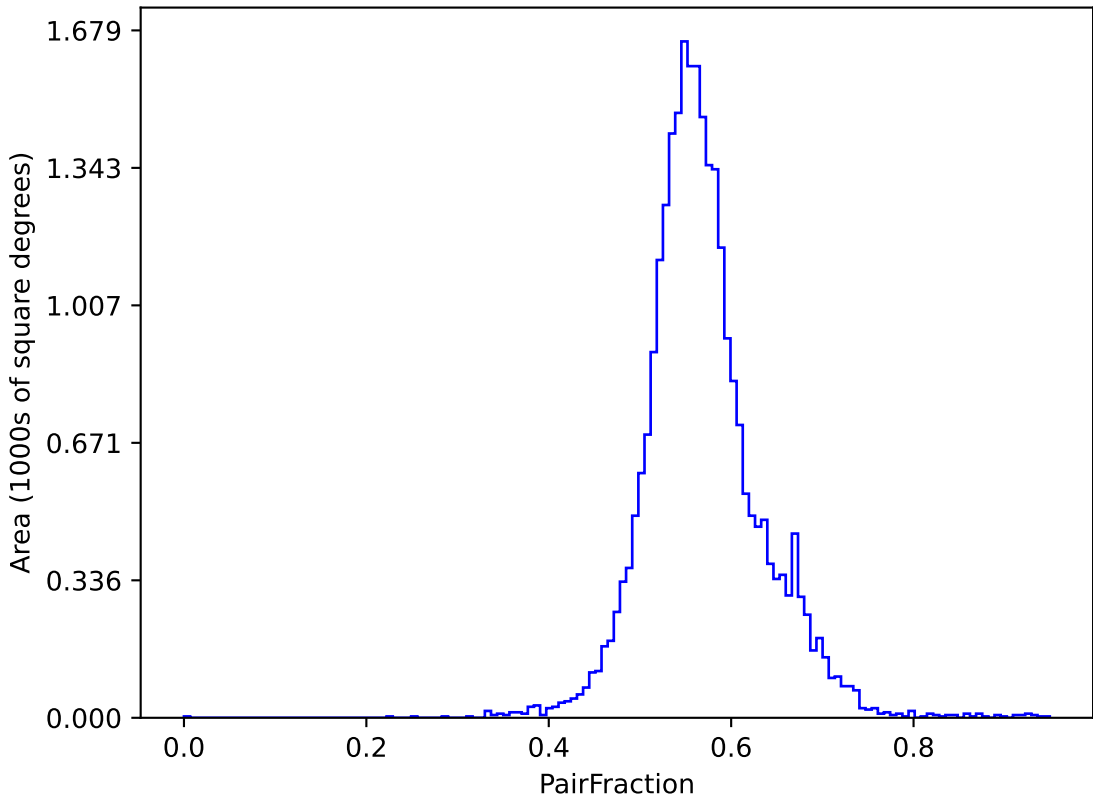
internal_u_expt27_nscale0.9v3.4_10yrs (g or r or i): PairFraction
