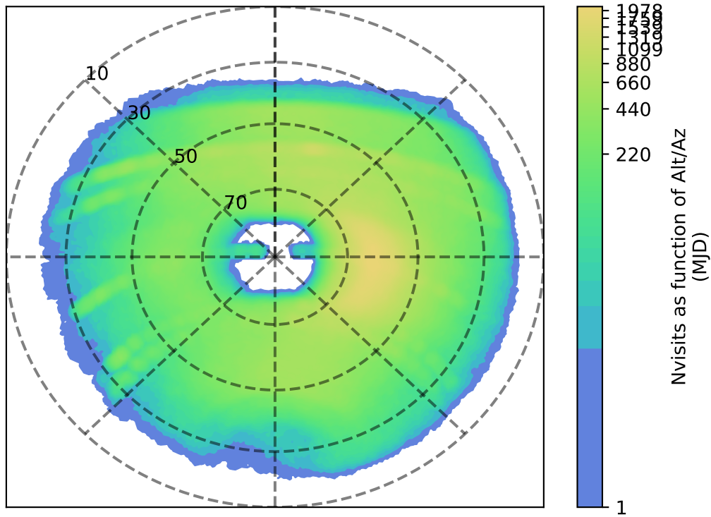
internal_u_expt27_nscale0.9v3.4_10yrs y: Nvisits as function of Alt/Az
