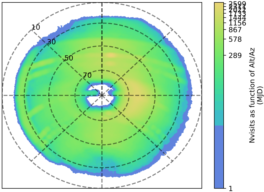
internal_u_expt27_nscale0.9v3.4_10yrs r: Nvisits as function of Alt/Az
