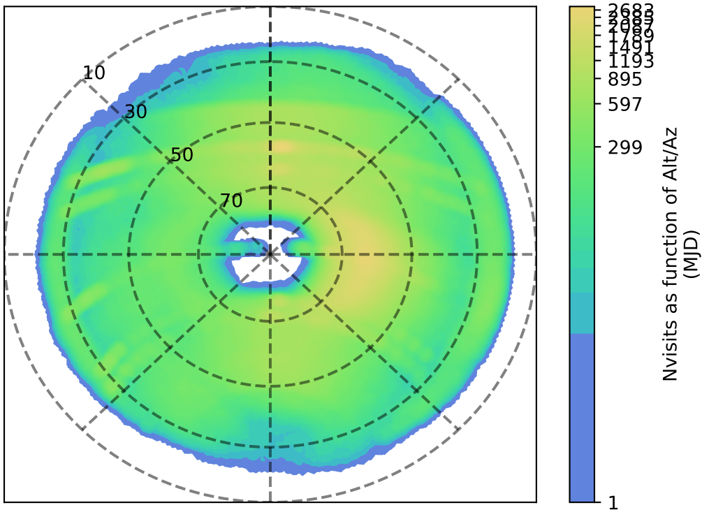
internal_u_expt27_nscale0.9v3.4_10yrs i: Nvisits as function of Alt/Az
