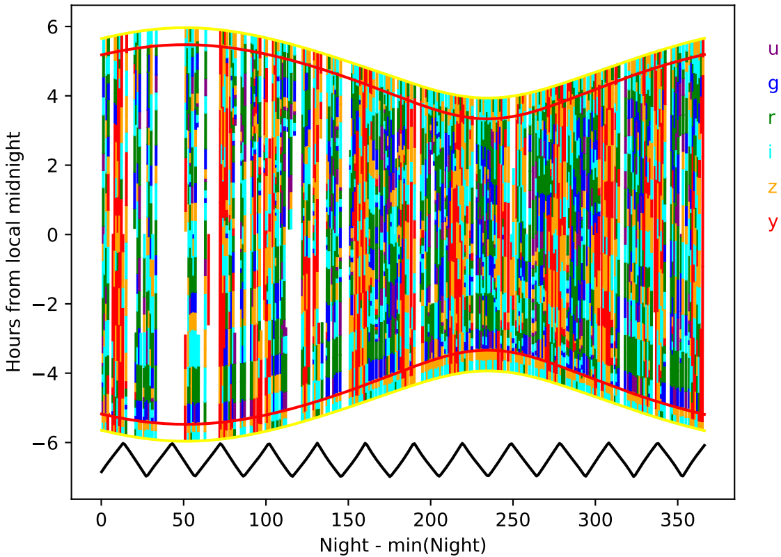
internal_u_expt27_nscale0.9v3.4_10yrs year 8-9: Hourglass
