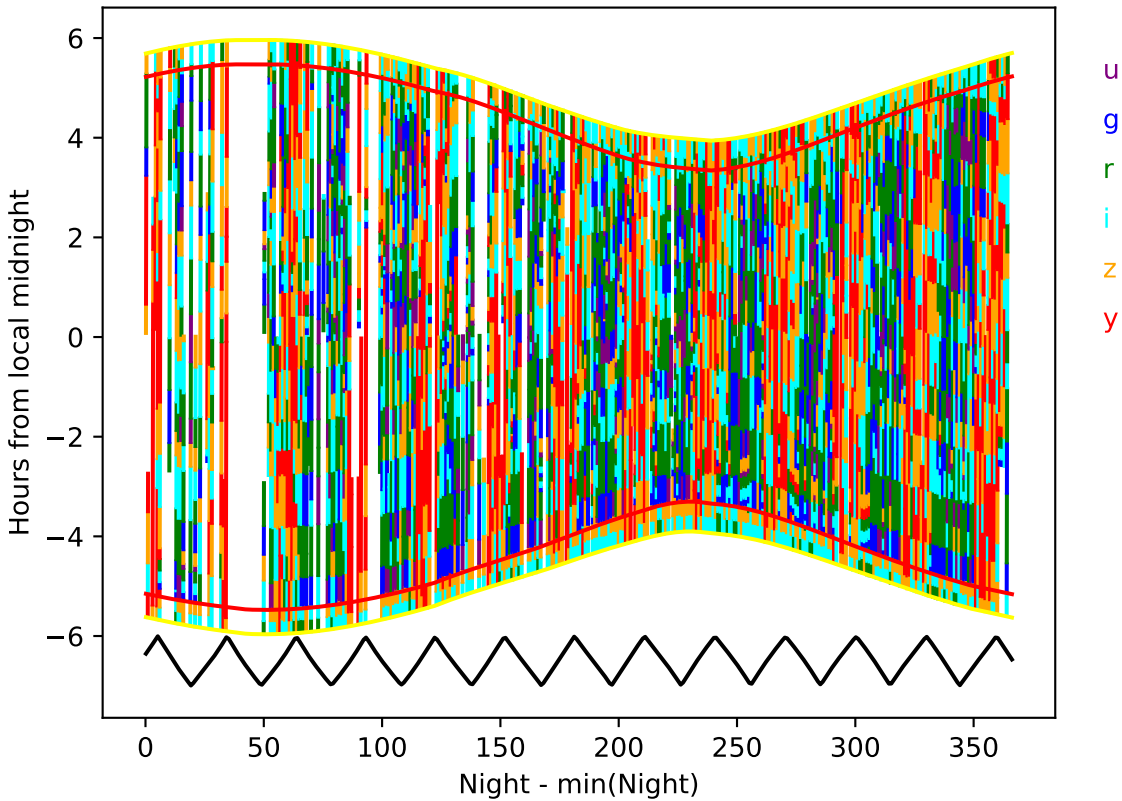
internal_u_expt27_nscale0.9v3.4_10yrs year 6-7: Hourglass
