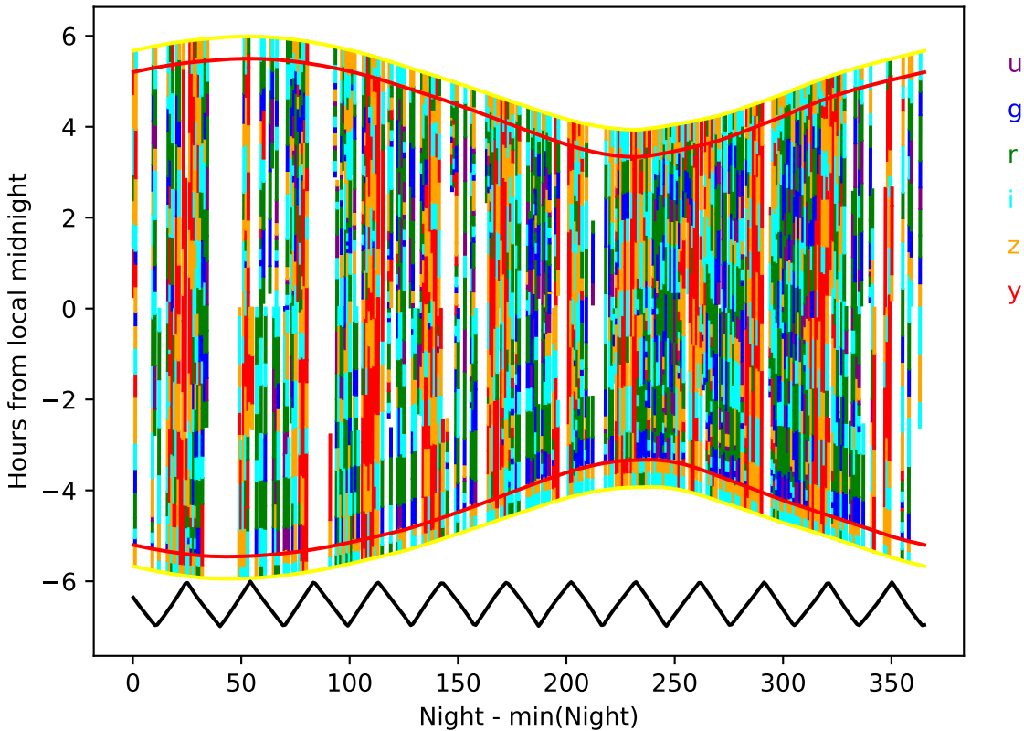
internal_u_expt27_nscale0.9v3.4_10yrs year 4-5: Hourglass
