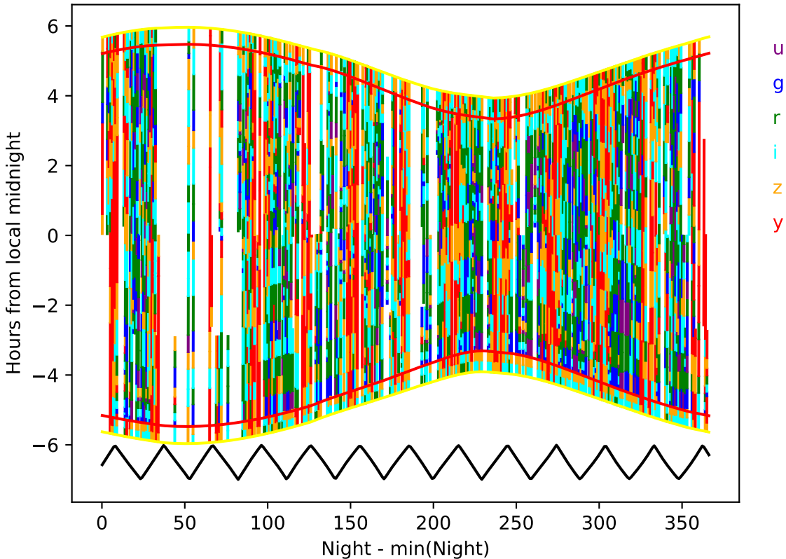
internal_u_expt27_nscale0.9v3.4_10yrs year 3-4: Hourglass
