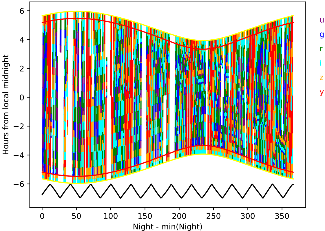
internal_u_expt27_nscale0.9v3.4_10yrs year 0-1: Hourglass
